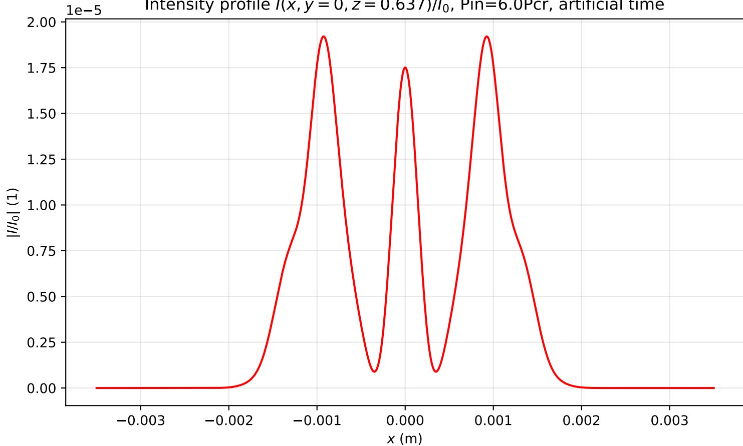
Intensity profile I(x, y = 0, z = 0.637)/I_0 , P_{in}=6.0P_{cr} , artificial time
